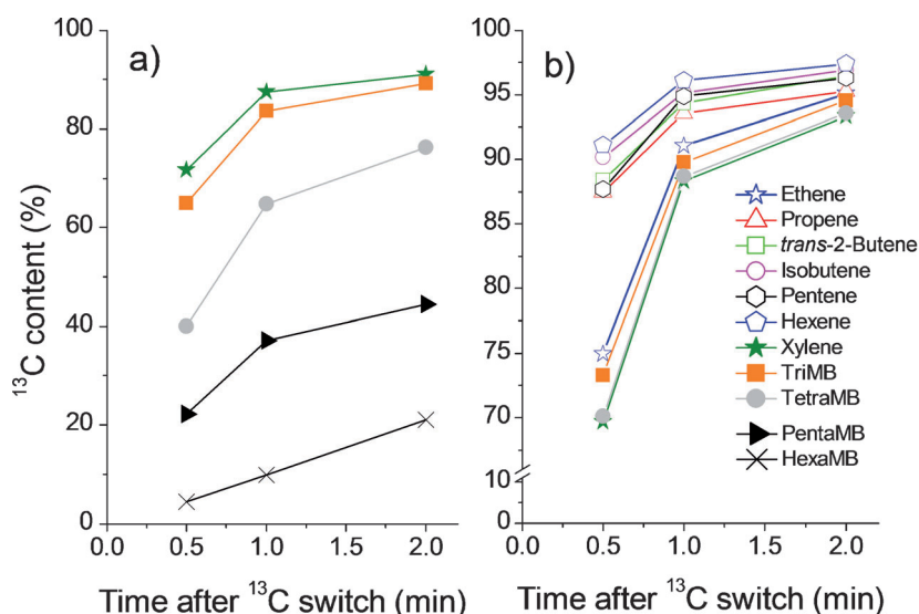
Figure 12. Transient ^{12}\text{C}/^{13}\text{C} methanol switch experiment carried out using H-ZSM-5 (Si/Al = 140). Methanol (WHSV = 7.0 \text{ g g}^{-1} \text{ h}^{-1} ) was reacted from the gas phase in a fixed-bed reactor at 350^\circ\text{C} . ^{12}\text{C} methanol was fed for 18 min before switching to ^{13}\text{C} methanol and reacting further for a predetermined time. The time evolution of ^{13}\text{C} content in effluent (b) and retained material (a) was determined from GC-MS analyses performed 0.5, 1.0, and 2.0 min after ^{12}\text{C}/^{13}\text{C} methanol feed switch. Adapted from Ref. [101].
