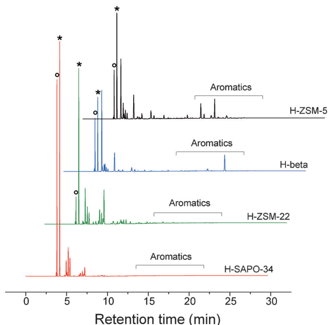
Figure 15. Chromatograms showing the MTH product distribution at 100% conversion over different catalysts; H-ZSM-5 (Si/Al = 50), H-beta (Si/Al = 45), H-ZSM-22 (Si/Al = 30), and H-SAPO-34 ((Al + P)/Si = 11). WHSV = 2 \text{ g g}^{-1} \text{ h}^{-1} and 400^\circ\text{C} . The ethene peaks are indicated by o and the propene by *. From Ref. [107].
