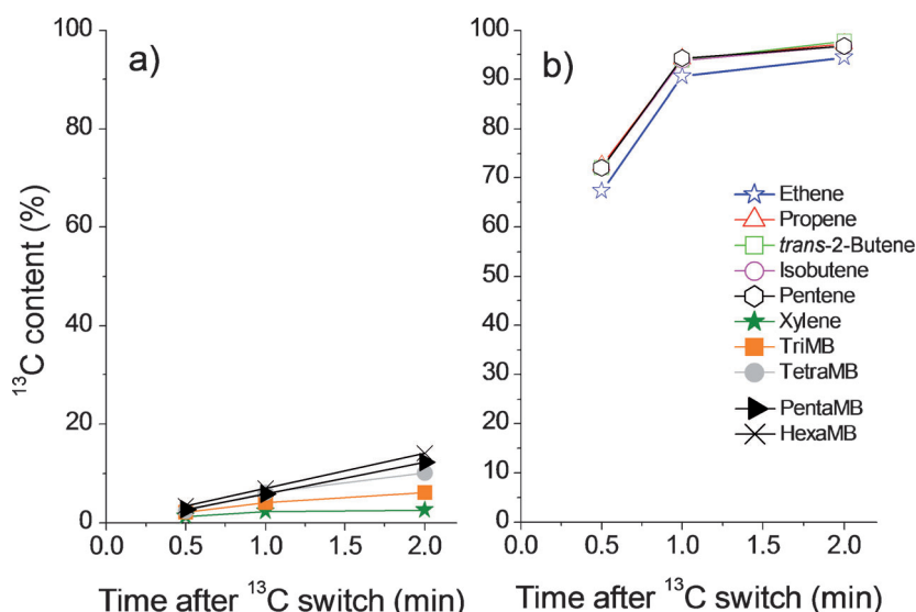
Figure 14. Transient ^{12}\text{C}/^{13}\text{C} methanol switch experiment carried out using H-ZSM-22 (Si/Al = 30). Methanol (WHSV = 2.0 \text{ g g}^{-1} \text{ h}^{-1} ) was reacted from the gas phase in a fixed-bed reactor at 400^\circ\text{C} . ^{12}\text{C} methanol was fed for 18 min before switching to ^{13}\text{C} methanol and reacting further for a predetermined time. The time evolution of ^{13}\text{C} content in effluent (b) and retained material (a) was determined from GC-MS analyses performed 0.5, 1.0, and 2.0 min after ^{12}\text{C}/^{13}\text{C} methanol feed switch. Adapted from Ref. [107].
