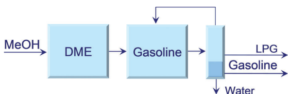
Figure 1. Methanol-to-gasoline (MTG) process: adiabatic dehydration reactor for DME synthesis and parallel adiabatic gasoline reactors. DME = dimethyl ether, LPG = liquified petroleum gas.
