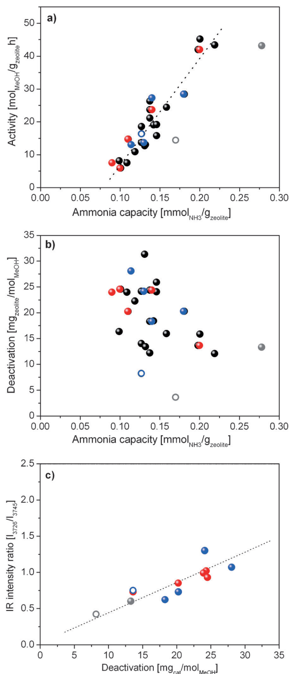
Figure 18. Influence of density of acid sites on a) MTH conversion and b) catalyst deactivation. c) The influence of the relative density of internal defects on catalyst deactivation for MTH reaction over H-ZSM-5 samples. From Ref. [21].
