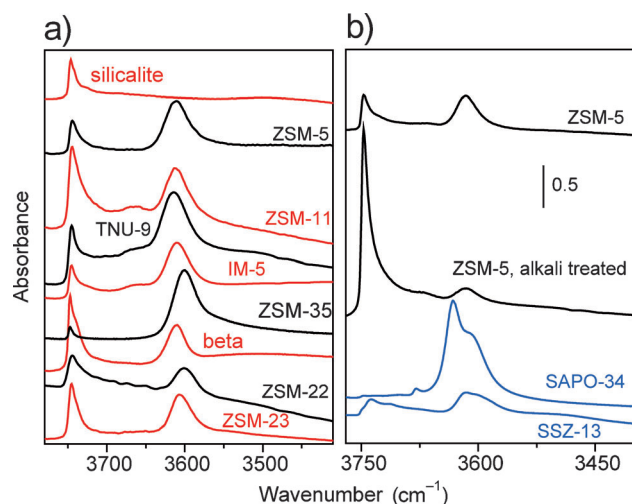
Figure 8. IR spectra of activated zeolites. a) From top to bottom: silicalite, H-ZSM-5, H-ZSM-11, H-TNU-9, H-IM-5, H-ZSM-35, H-Beta, H-ZSM-22 and H-ZSM-23. b) From top to bottom: H-ZSM-5, alkali-treated H-ZSM-5, H-SAPO-34, H-SSZ-13.
